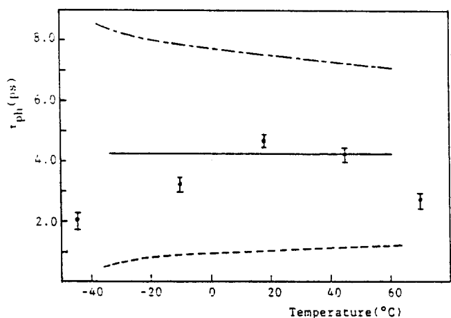
Figure 1. Temperature dependence of the dephasing time of \text{CH}_3\text{CN} . Experimental values from Ref. 25 ( \blacklozenge ), the Enskog theory (-----), the hydrodynamic theory (.....), and the theory of Sung and Stell (——).
