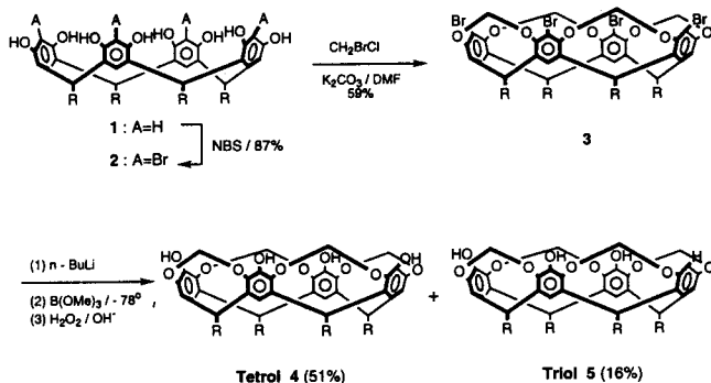
Scheme 1. Synthesis of Solubility-Increased Tetrol 4 and Triol 5 ( R=(\text{CH}_2)_{10}\text{CH}_3 ).
