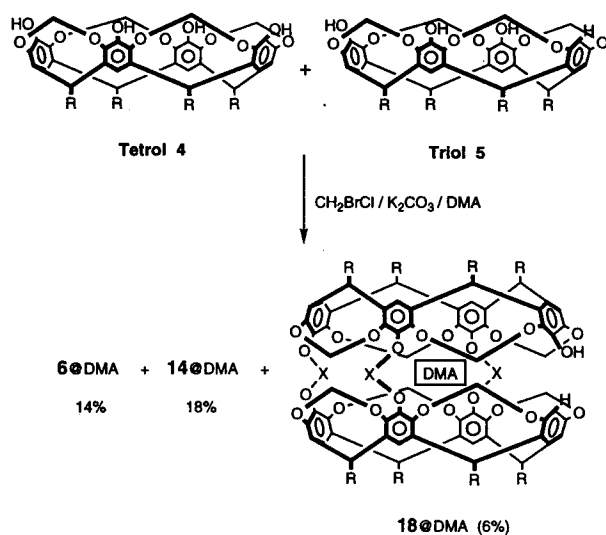
Scheme 5. One-Pot Synthesis of Three Container Hosts 6 , 14 , and 18 Having DMA ( R=(CH_2)_{10}CH_3 ).
