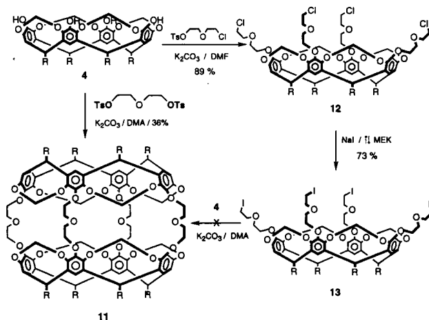
Scheme 3. Synthetic Route of Hemicarcerand 11 ( R=(\text{CH}_2)_{10}\text{CH}_3 ).
