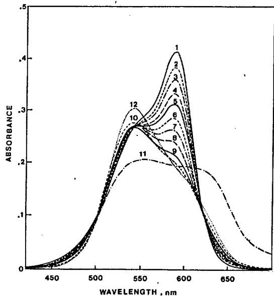
Figure 2. Absorption spectra of CV + and its ion aggregates with TFB - at pH=5.0 and \mu=0.01M . [CV + ]= 4.0 \times 10^{-6}M , [TPB - ], 10^{-6}M : (1) 0.0; (2) 0.4; (3) 0.8; (4) 1.2; (5) 1.6; (6) 2.0; (7) 2.4; (8) 2.8; (9) 3.2; (10) 3.6; (11) 4.0; (12) 400.
