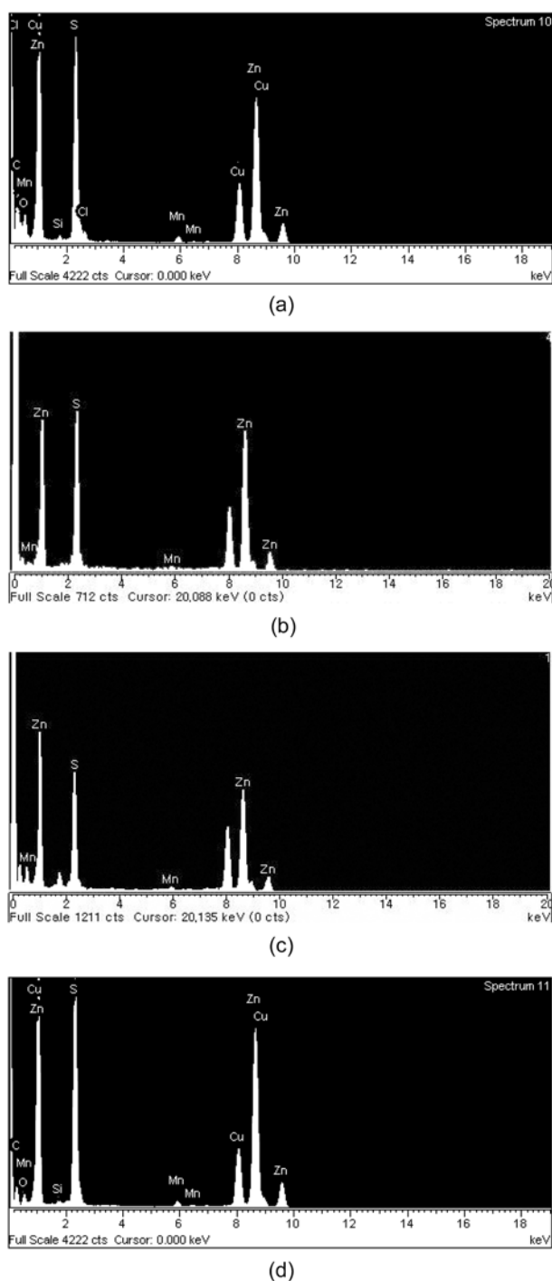
Figure 4. EDXS spectra for the aminoacids capped ZnS:Mn nanocrystals. (a) EDXS spectrum of ZnS:Mn (Arg) nanocrystal. (b) EDXS spectrum of ZnS:Mn (Cys) nanocrystal. (c) EDXS spectrum of ZnS:Mn (His) nanocrystal. (d) EDXS spectrum of ZnS:Mn (Met) nanocrystal.
