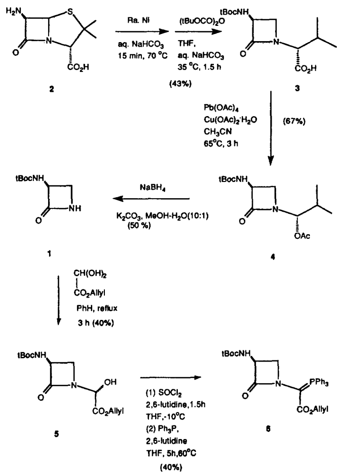
Scheme 1.
