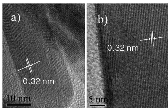
Figure 2. HRTEM photographs of \text{Gd}(\text{OH})_3:\text{Eu} prepared by hydrothermal reaction at 180 °C. pH = (a) 12.9 (nanorods) and (b) 10.8 (nanowires).
