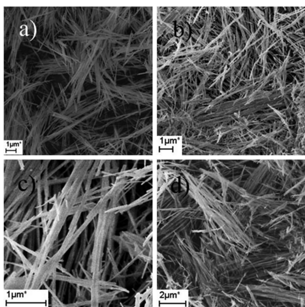
Figure 7. FE-SEM photographs of (a) \text{Gd}(\text{OH})_3\text{:Eu} prepared by hydrothermal reaction at 180 °C, pH = 12.1 and \text{Gd}_2\text{O}_3\text{:Eu} obtained after dehydration at (b and c) 500 °C and (d) 800 °C.
