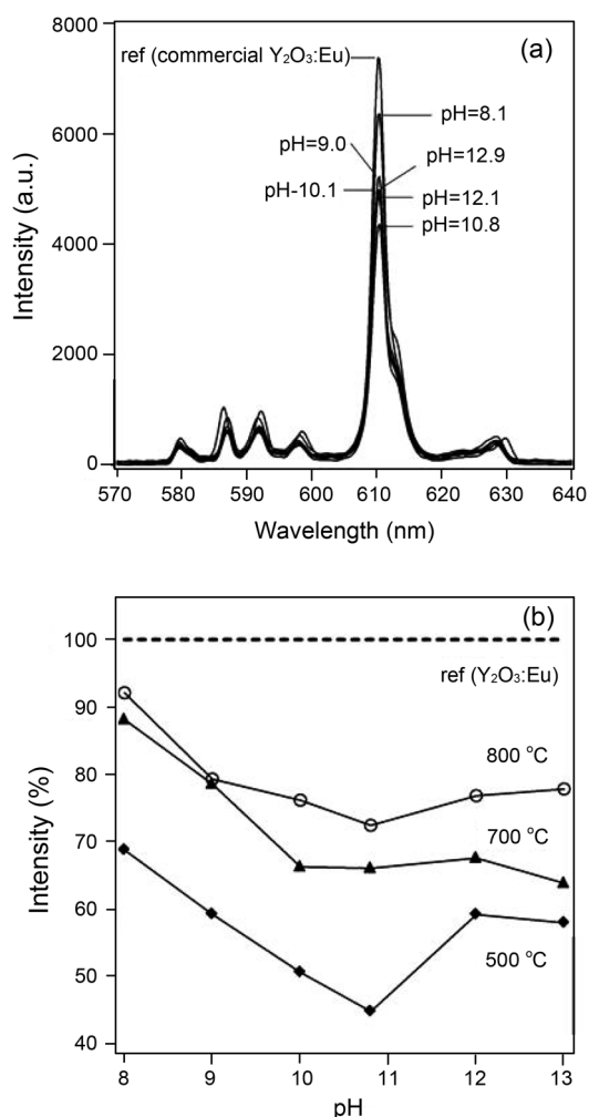
Figure 9. (a) PL emission spectra of \text{Gd}_2\text{O}_3\text{:Eu} obtained after dehydration of \text{Gd}(\text{OH})_3\text{:Eu} at 800 °C. PL emission spectrum of commercial \text{Y}_2\text{O}_3\text{:Eu} is also compared as a reference. (b) Comparison of the relative PL emission intensity of \text{Gd}_2\text{O}_3\text{:Eu} phosphors obtained after heat treatment for 5 h as a function of the solution pH for the hydrothermal synthesis. All intensities were measured as values relative to that of commercial \text{Y}_2\text{O}_3\text{:Eu} .
