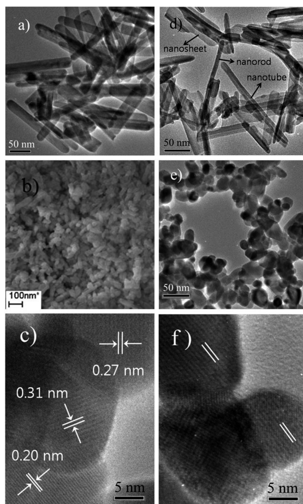
Figure 8. FE-SEM and TEM photographs of (a) \text{Gd}(\text{OH})_3\text{:Eu} prepared by hydrothermal reaction at 180 °C, pH = 12.9 and (b and c) \text{Gd}_2\text{O}_3\text{:Eu} obtained after dehydration at 500 °C. TEM photographs of (d) \text{Gd}(\text{OH})_3\text{:Eu} prepared at 120 °C, pH = 12.9 and (e and f) \text{Gd}_2\text{O}_3\text{:Eu} obtained after dehydration at 500 °C.
