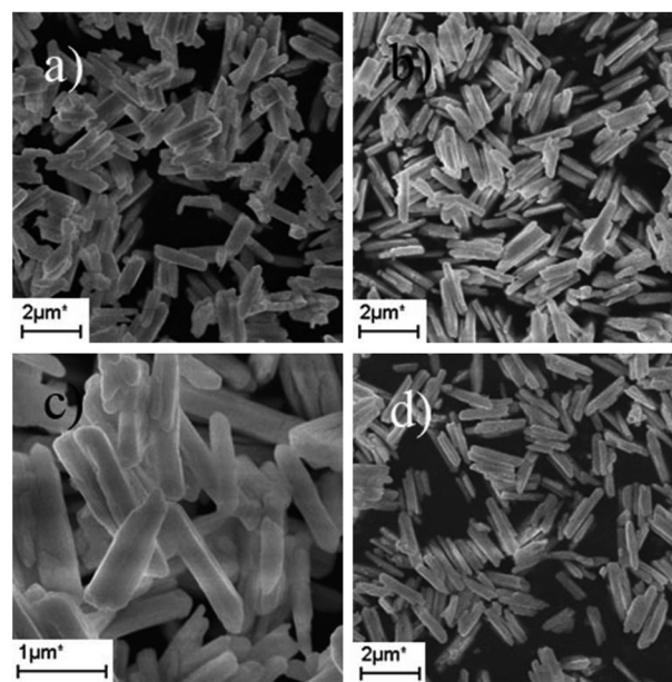
Figure 3. FE-SEM photographs of (a) \text{Gd}(\text{OH})_3:\text{Eu} prepared by hydrothermal reaction at 180 °C, \text{pH} = 8.1 and \text{Gd}_2\text{O}_3:\text{Eu} obtained after dehydration at (b and c) 500 °C and (d) 800 °C.
