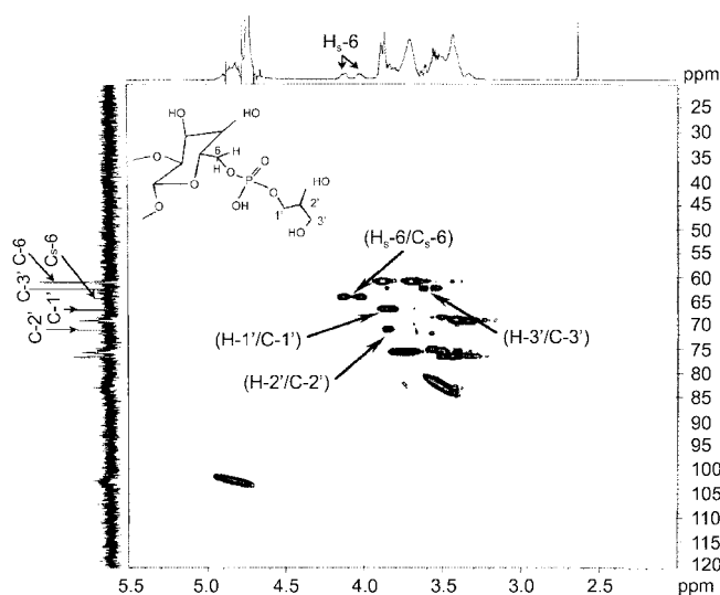
Figure 2. HSQC spectrum of anionic cyclosophoraoses. sn -glycerol-1-phosphate residues were directly linked to the C-6 of glucose residue through a phosphodiester linkage. ( C_s -6 and H_s -6: C-6 and H-6 of the glucose residue substituted with glycerol-1-phosphate).
