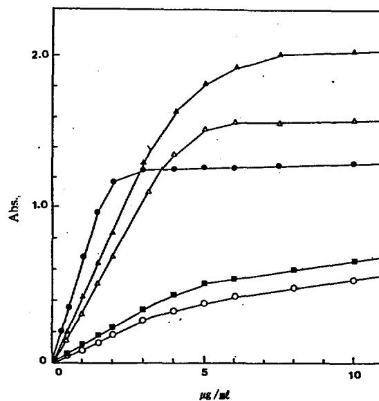
Figure 3. Maximum adsorption of each metal on concentrator column. ○; Fe(II), △; Cu(II), ▲; Ni(II), ■; Zn(II), ●; Co(II).
