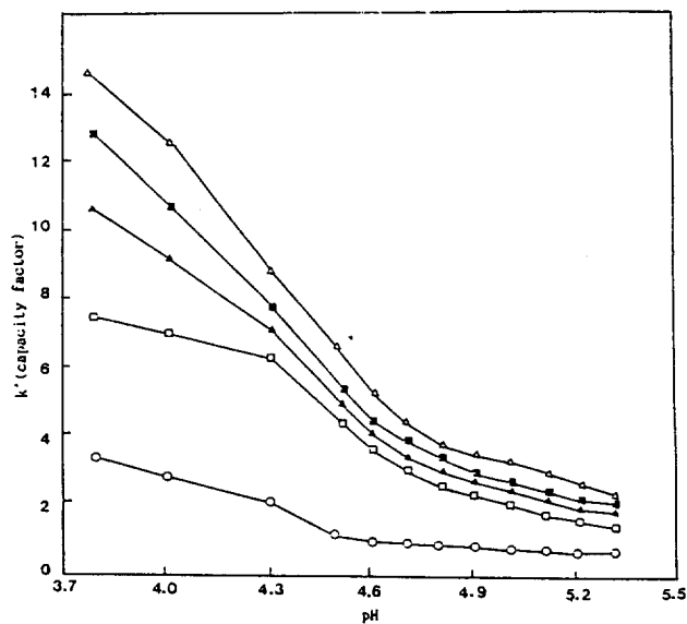
Figure 5. Variation of capacity factor as a function of the eluent pH. \circ ; Fe(III), \square ; Cu(II), \blacktriangle ; Ni(II), \blacksquare ; Zn(II), \triangle ; Co(II).
