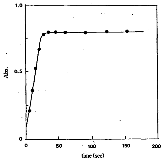
Figure 2. Effect of pumping time on on-column pre-concentration.
