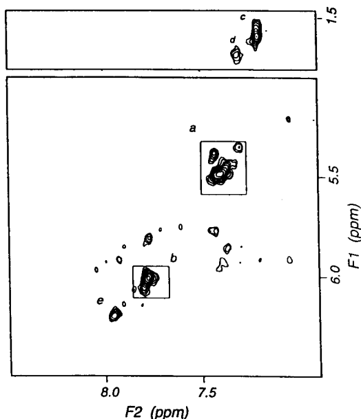
Figure 3. The crosspeak region between aromatic and sugar H1' proton resonances of NOESY spectrum of Co-form of the TA 14 mer in D 2 O at 35 °C and \tau_m=300 ms. 512 t_1 values of 64 scans each were collected. The spectrum was zero-filled in t_1 and apodized with a squared sinebell phase shifted by 90° in both dimensions. (a) and (b) are overlapped crosspeaks between C-H5 and C-H6. (c) and (d) are crosspeaks between T-5Me and T-H6 of both B-form and Z-form. Samples are the same as Figure 2.
