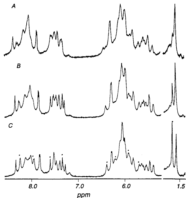
Figure 2. ^1H NMR spectra of the aromatic and the T methyl proton resonances of the Co-form of the TA 14 mer in 20 mM NaCl and 2 mM Co(NH_3)_6Cl_3 , pH 7.0, D_2O at (A) 30 °C, (B) 40 °C, (C) 50 °C. New resonances are marked by * in (C).
