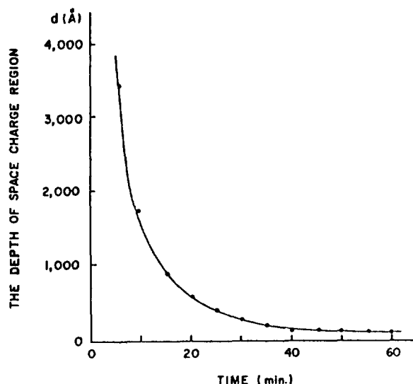
Figure 1. Variation of the apparent depth of space charge region of ZnO (10 \bar{1}0 ) depend on evacuation time at 773 K.
