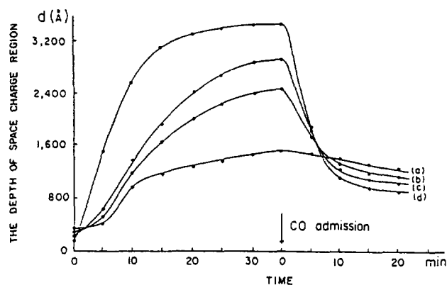
Figure 3. Effect of admission of oxygen (400 N/m 2 ) and carbon monoxide (2660 N/m 2 ) on the apparent depth of space charge region of ZnO (10 \bar{1}0 ) at 373 K (a), 473 K (b), 573 K (c) and 673 K (d).
