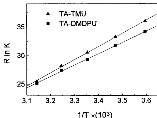
Figure 3. The van't Hoff plot for the TA:TMU and TA:DMDPU 1:1 complex formation.
