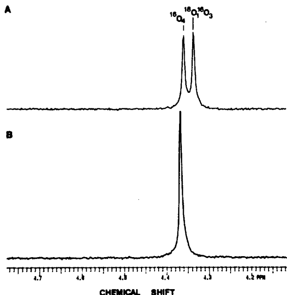
Figure 4. 31 P-NMR spectrum of the AMP product of the 18 O transfer experiment. (Panel A) AMP product. The relative integrals of the peaks are 0.96 and 1.00 (Panel B) Standard AMP.
