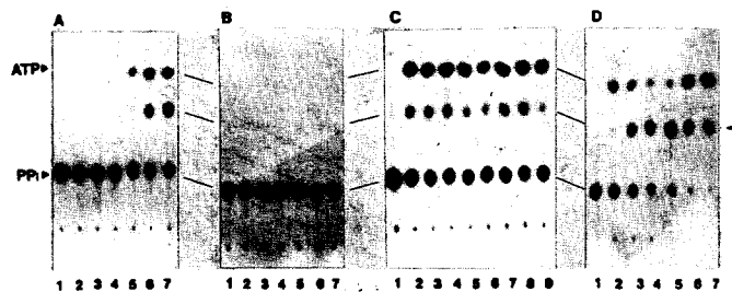
Figure 5. Autoradiogram of TLC analysis of reaction products using [ α- 32 P ]ATP. The basic reaction mixtures contained 0.1 M potassium phosphate (pH 7.1) buffer, 5 μM MgCl 2 , 0.2 pmol [ α- 32 P ]ATP, other components in the indicated amount, and 7.5 × 10 -3 unit of malonyl-CoA synthetase (6 pmol) in a total volume of 25 μl. All other conditions are as described in the legend of Figure 3. (Panel A) Lane 1, control (with boiled enzyme); lane 2-4, 1 min, 4 min, and 8 min in reaction with only [ α- 32 P ]ATP as a substrate, respectively; lane 5-7, 1 min, 4 min, and 8 min after subsequent addition of malonate to final concentration of 2 mM, respectively. (Panel B) The explanation for each lanes are the same as described in panel A except for the addition of 2 mM succinate in place of malonate. (Panel C) The basic reaction mixtures were first incubated for 8 min at 37°C. Malonate (final concentration, 2 μM) and inhibitor (in the indicated concentration) mixed previously were added and the mixtures were quickly mixed with a vortex mixer. The incubation was continued for 8 min at 37°C. Lane 1, control (with boiled enzyme); lane 2, only malonate without inhibitor; lane 3-6, 0.1 μM, 1 μM, 10 μM, and 100 μM AMP respectively; lane 7-9, 0.2 mM, 2 mM, and 20 mM succinate respectively. (Panel D) The basic reaction mixtures contained [ α- 32 P ]ATP and malonate (final concentration of 1 mM) as substrates. After 4 min, aliquots of 10 ml were taken and mixed with CoA (final concentration of 0.5 mM). The mixture containing CoA was separately incubated and aliquots of 1 μl were spotted onto a PEI-cellulose plate at the indicated time. Lane 1, control (with boiled enzyme); lane 2-5, 1 min, 4 min, 8 min, and 12 min from the reaction mixture in the absence of CoA, respectively; lane 6-7, 4 min and 8 min after the addition of CoA, respectively. The positions of each nucleotides were identified using unlabelled ATP, ADP, and AMP. The arrow indicates the novel nucleotide derivative, defined as malonyl-AMP.
