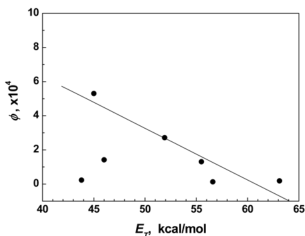
Figure 6. The luminescence quantum yield of [Ru(phen) _2 BDPPZ] ^{2+} with respect to the polarity of solution. From left to right on the x -axis, the solutions were DMF, DMSO, MeCN, ethanol, methanol, formamide and water.
