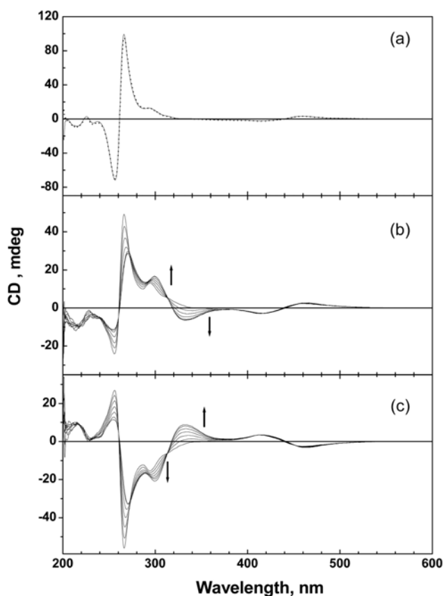
Figure 5. CD spectrum of \Lambda -[Ru(phen) _3 ] ^{2+} (panel (a)), \Lambda -[Ru(phen) _2 BDPPZ] ^{2+} (panel(b)), and \Delta -[Ru(phen) _2 BDPPZ] ^{2+} (panel(c)) in the presence of poly(dT). [Ru(II) complex] = 5 \mu M. In panel (a), the CD spectra of \Lambda -[Ru(phen) _3 ] ^{2+} in the absence (solid curve) and presence of 12 \mu M poly(dT) (dotted curve) are compared. In Panel (b) and (c), the concentration of poly(dT) increases gradually in the direction of the arrow. [Poly(dT)] = 2, 4, 6, 8, 10, 12 \mu M.
