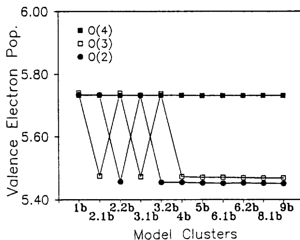
Figure 11. Valence electron populations for each site of oxygen 2p orbitals in the charged model clusters representing \text{YBa}_2\text{Cu}_3\text{O}_6 .
