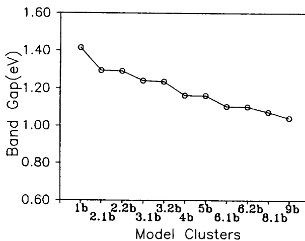
Figure 6. Band gap between the bottom of the cluster x^2-y^2 Cu(2) band and the top of the cluster z^2 Cu(1) band for the charged model clusters representing YBa_2Cu_3O_6 .
