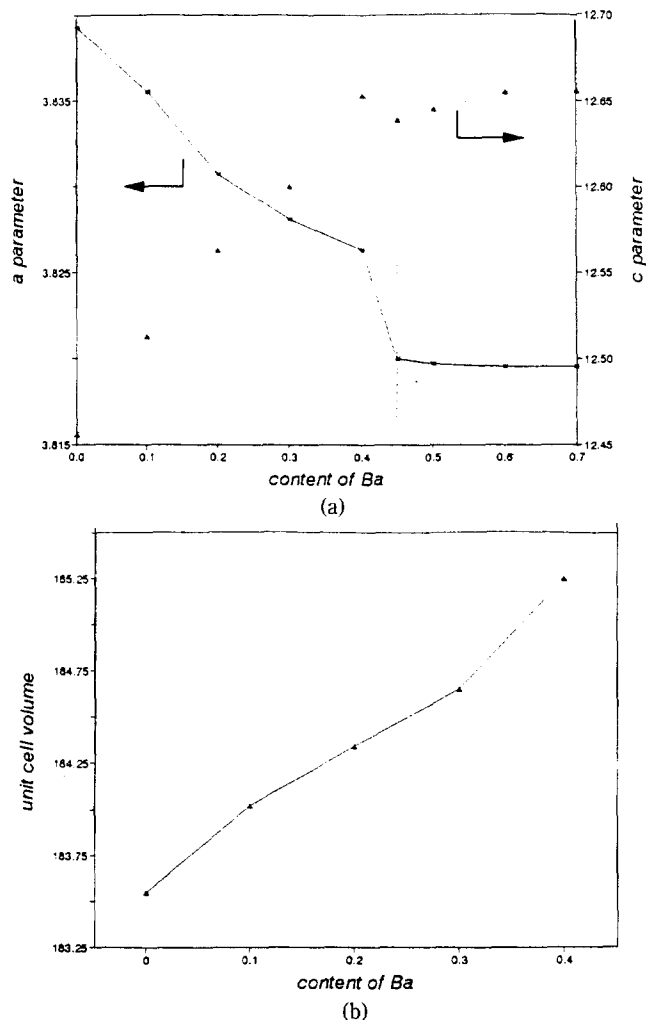
Figure 2. The variations of a) a - and c -parameters, and b) unit cell volume as a function of the Ba content ( x ) of \text{Pr}_{2-x}\text{Ba}_x\text{NiO}_{4+\delta} . Data points for x < 0.5 are for sample obtained from 1300 °C reaction and the rest are from 1200 °C.
