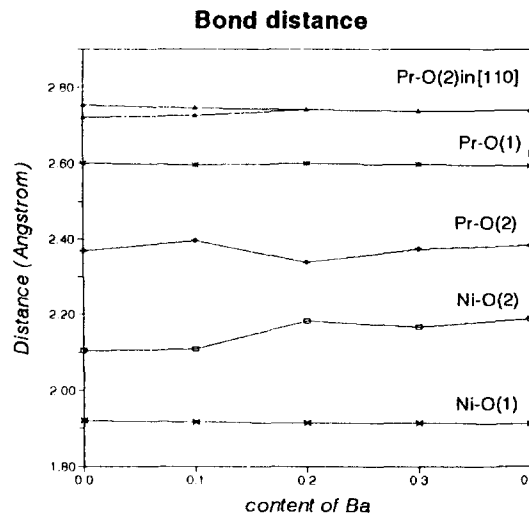
Figure 3. Variations of Ni-O and Pr(Ba)-O bond distances in the \text{Pr}_{2-x}\text{Ba}_x\text{NiO}_4 system.
