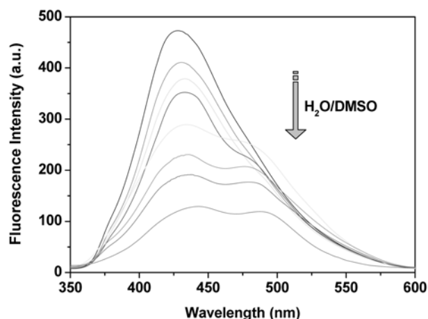
Figure 1. Fluorescence spectra of 1 (5.0 μM) in H 2 O/DMSO mixture with an excitation at 335 nm. Ratios of H 2 O/DMSO: DMSO only, 1/4, 3/7, 2/3, 1/1, 3/2, 7/3 and 4/1.
