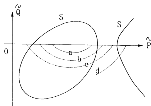
Figure 3. A schematic diagram of solutions of 20-moment equations in the phase space. The curve S represents a contour line of \tilde{R}^{(p)}=0 of the singular surface. The dotted curves are projections of hypothetical loci of solution points onto the (\tilde{P}, \tilde{Q}) plane in the phase space.
