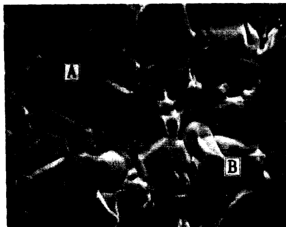
Figure 2. A typical SEM photograph of 8.0% MgO-Fe _2 O _3 . A: Mg _3-x O _4 B: \alpha -Fe _2 O _3
