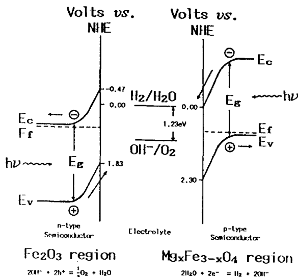
Figure 6. Energy level diagram for depicting band edge locations of 8.0% MgO doped Fe 2 O 3 relative to hydrogen/oxygen redox couples.
