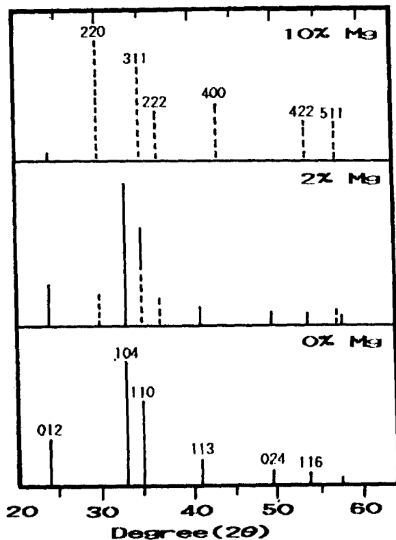
Figure 1. Typical X-ray diffraction patterns(CuK \alpha ) for MgO doped Fe _2 O _3 disks, —; full solid line means a corundum phase; ·····; dotted line means a spinel phase.
