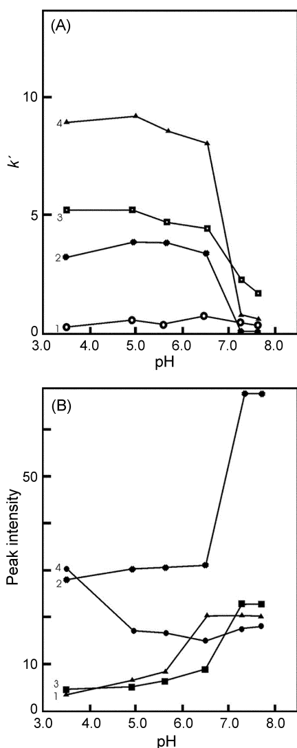
Figure 2. The effect of pH for the k' (A) and peak intensity (B) of the compounds on C_4 at 15 °C. a Concentration of the compounds; [TAR] & [5MTAR]; 1.4 \times 10^{-4} M, [Co(II)-TAR]; 1.0 \times 10^{-5} M, [Co(II)-5MTAR]; 2.0 \times 10^{-5} , Identification; 1: Co(II)-TAR, 2: TAR, 3: Co(II)-5MTAR, 4: 5MTAR, Mobile phase: 22.5% MeCN.
