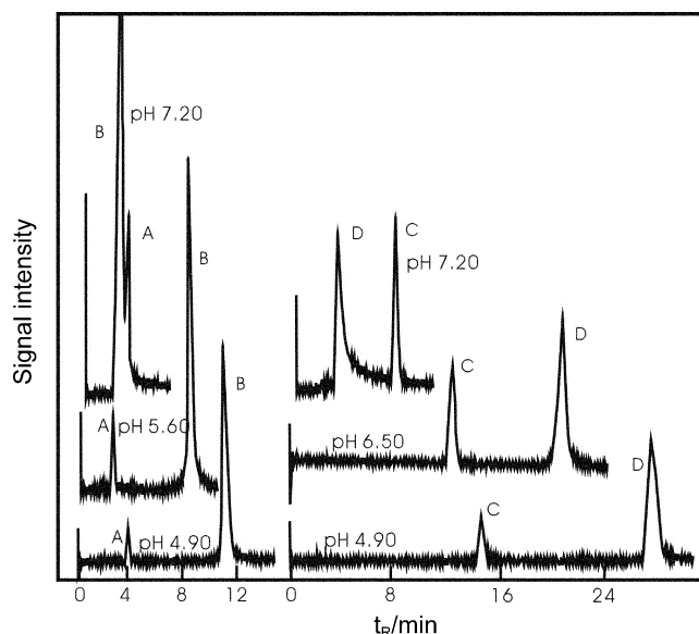
Figure 3. Separation chromatograms of Co(II)-TAR and TAR, and Co(II)-5MTAR and 5MTAR by using 22.5% (v/v) MeCN as mobile phase at various pH. a Column, MeCN percentage in mobile phase, concentration of each compounds in sample solutions, and temperature are same as in Figure 2, Identification; A: Co(II)-TAR, B: TAR, C: Co(II)-5MTAR, D: 5MTAR.
