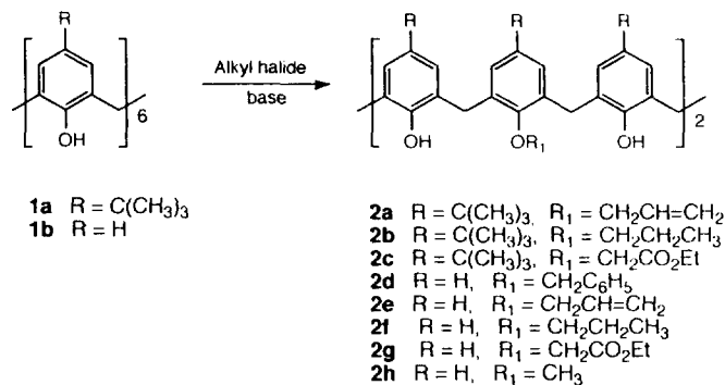
Scheme 1. Dialkylation of Calix[6]arene.
