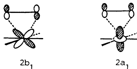
Figure 9 shows a Walsh diagram as a function of r . Among various orbitals, two orbitals derived from 2a_1 and
