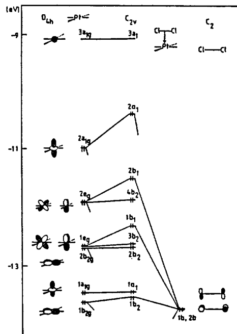
Figure 8. Correlation diagram of orbitals of \text{Pt}(\text{CN})_4\text{Cl}_2 with D_{4h} \text{Pt}(\text{CN})_4 and C_{2v} \text{Cl}_2 .
