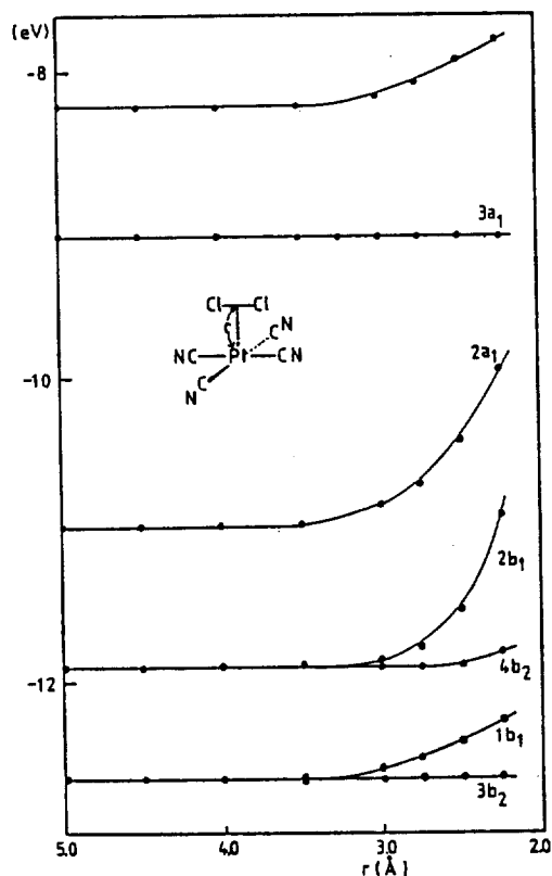
Figure 9. Walsh diagram of a C_{4v} \text{Pt}(\text{CN})_4\text{Cl}_2 fragment as a function of r , with fixed Cl-Cl distance.
