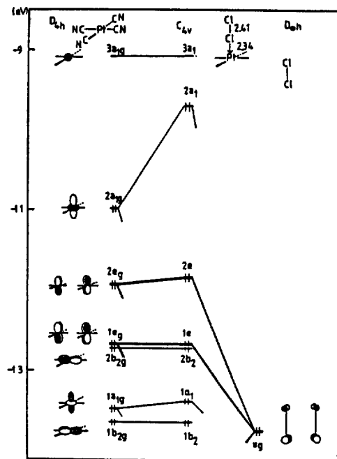
Figure 2. Correlation diagram of orbitals of \text{Pt}(\text{CN})_4\text{Cl}_2 with D_{4h} \text{Pt}(\text{CN})_4 and D_{oh} \text{Cl}_2 .
