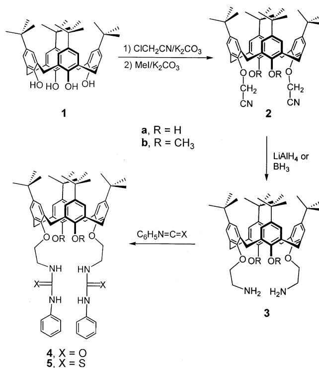
Scheme 1. Synthesis of Urea Derivatized Calix[4]arenes.
