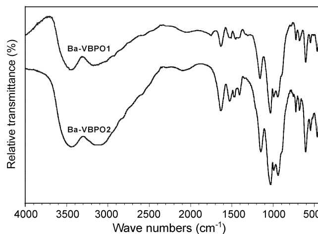
Figure 1. IR spectra of Ba-VBPO1 and Ba-VBPO2 .
