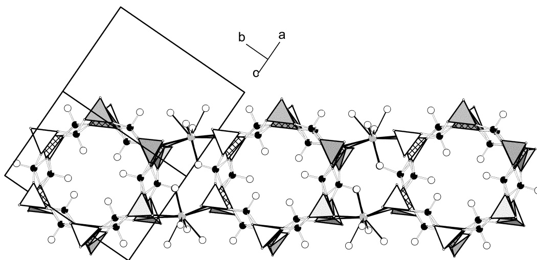
Figure 3. View along [101] direction showing the infinite chain in Ba-VBPO1 . The PO 4 and BO 4 units are shown as filled and crosshatched tetrahedra, vanadium, oxygen and barium atoms as filled, open and gray circles, respectively.
