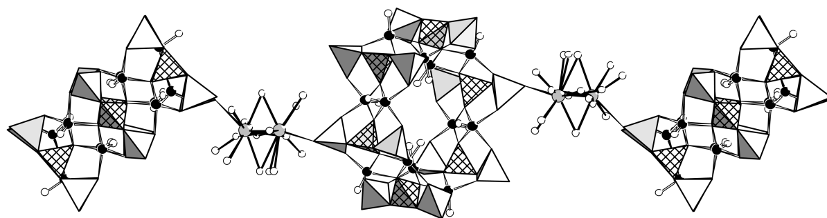
Figure 4. View of Ba-VBPO2 showing the connectivity between [(\text{NH}_4) \supset \text{V}_2\text{P}_2\text{BO}_{12}]_6 cluster anions and \text{Ba}^{2+} cations, which are disordered over two positions. The \text{PO}_4 and \text{BO}_4 units are shown as filled and crosshatched tetrahedra, vanadium, oxygen and barium atoms as filled, open and gray circles, respectively.
