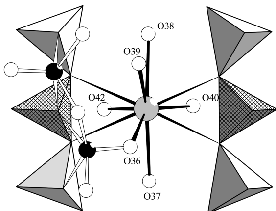
Figure 2. Connectivity of Ba atom and two [(NH 4 ) 2 V 2 P 2 BO 12 ] 6 cluster anions for Ba-VBPO1 . Parts of the cluster anions are shown for clarity. The PO 4 and BO 4 units are shown as filled and crosshatched tetrahedra, vanadium and oxygen atoms as filled and open circles, respectively and a barium atom as a gray circle.
