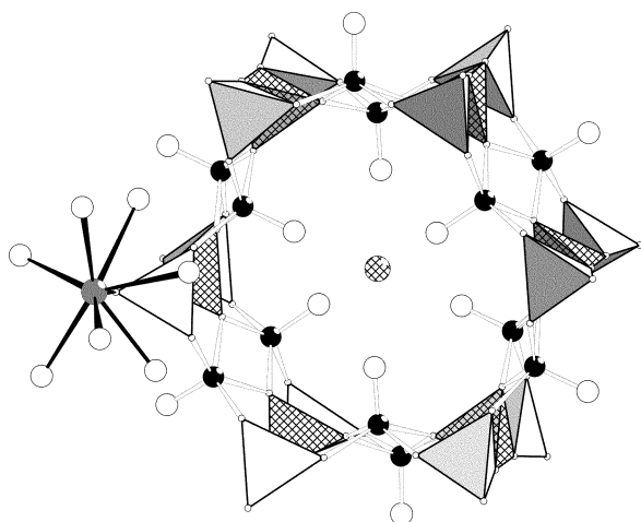
Figure 5. [\text{Ba}(\text{H}_2\text{O})_7][(\text{NH}_4) \supset \text{V}_2\text{P}_2\text{BO}_{12}]_6 cluster anion in Ba-VBPO2 . The \text{PO}_4 and \text{BO}_4 units are shown as filled and crosshatched tetrahedra, vanadium and oxygen atoms as filled and open circles, and a barium and nitrogen atom as a gray and crosshatched circles, respectively.
