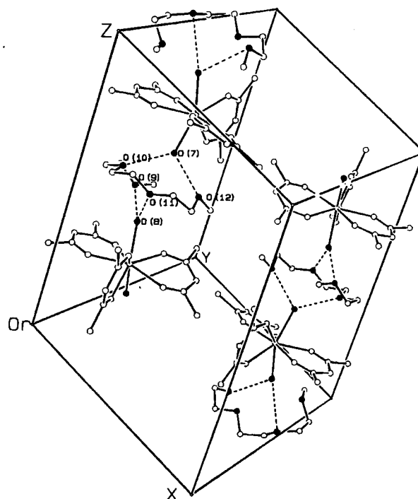
Figure 2. Unit cell packing diagram showing the chains running along the z axis.
