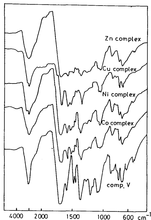
Figure 2. Infrared spectra of N-phenylphthalimide and its metal complexes.
