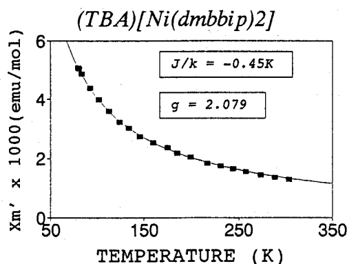
Figure 3. Temperature dependence of magnetic susceptibility ( \chi_m' ) for (TBA)[Ni(dmbbip) 2 ]. The solid line represents a fit to the calculated series expansion for a two-dimensional Heisenberg-antiferromagnet system.
