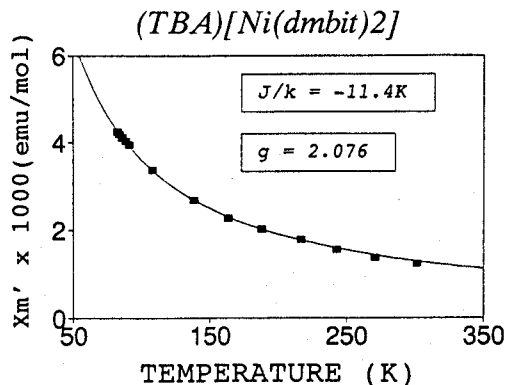
Figure 2. Temperature dependence of magnetic susceptibility ( \chi_m' ) for (TBA)[Ni(dmbit) 2 ]. The solid line represents a fit to the calculated series expansion for a two-dimensional Heisenberg-antiferromagnet system.
