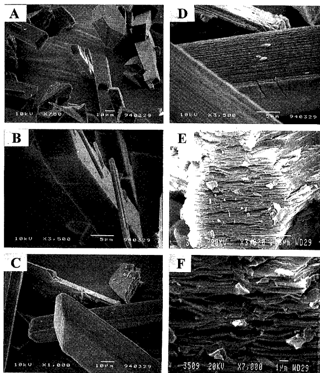
Figure 1. SEM images of (TBA) 2 [Ni(dmbit) 2 ] (A and B), (TBA)[Ni(dmbit) 2 ] (C and D) and (TBA)[Ni(dmbbip) 2 ] (E and F).
