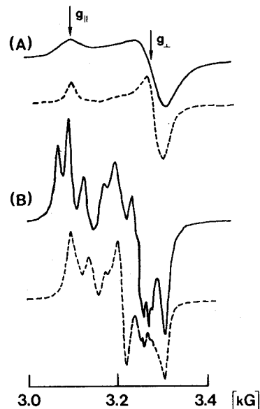
Figure 4. X-band EPR spectra of polycrystalline (A) (TBA)[Ni(dmbit) 2 ] and (B) (TBA)[Ni(dmbbip) 2 ] at 300 K (solid line) and 77 K (broken line), respectively.
