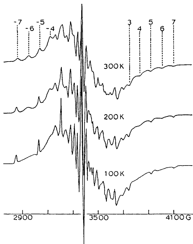
Figure 1. Temperature variation of the polycrystalline EPR spectrum of \alpha -1,2,3-[H 2 PV(IV)V 2 W 6 O 40 ] 5- doped into K 5 [H 2 SiV 3 W 6 O 40 ]. Parallel lines are designated by the m_i values of an I=7 system. Microwave frequency: 9.4394 GHz.
