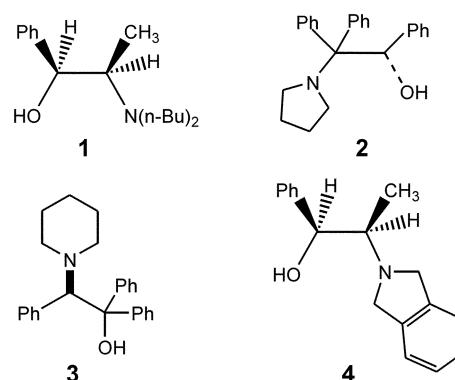
Figure 1. \beta -Aminoalcohols for diethylzinc addition.
