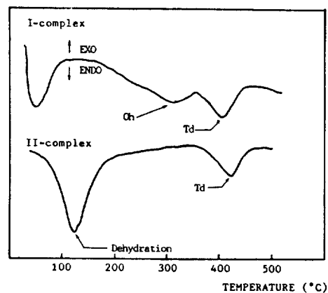
Figure 1. DSC curves of n -hexylammonium-layer silicate complexes with heating rate of 10^\circ\text{C}/\text{min} under nitrogen atmosphere.
