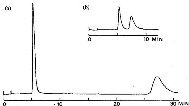
Figure 1. Chromatograms for resolving 4c on (a) CSP 1 and on (b) CSP 2 . For chromatographic conditions, see the footnote to Table 1.
