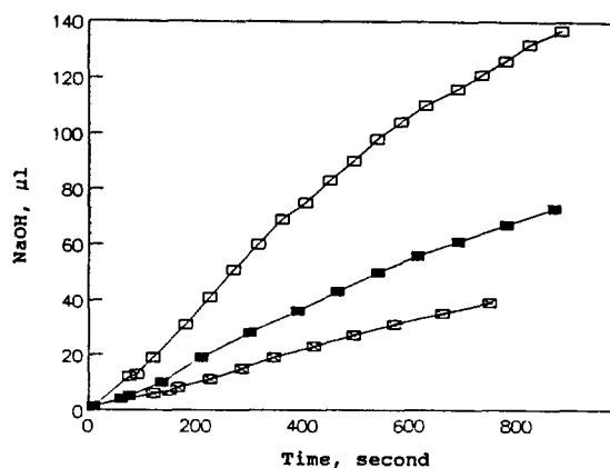
Figure 1. Time dependence of the amount of NaOH added in the hydrolysis of PC LUV system by PLD. The incubation medium contained 10 mM \text{CaCl}_2 , 10^{-5} M DTT, and 2.64 mM PC. \square , 7.5 \mu\text{g} of protein; \blacksquare , 3.9 \mu\text{g} of protein; \circ , 1.9 \mu\text{g} of protein.
