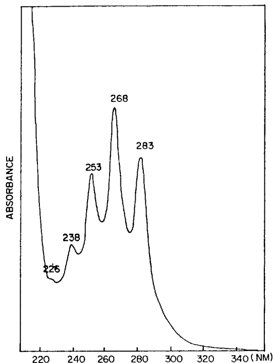
Figure 1. UV Spectrum of C-1 Polyacetylene (in MeOH).
