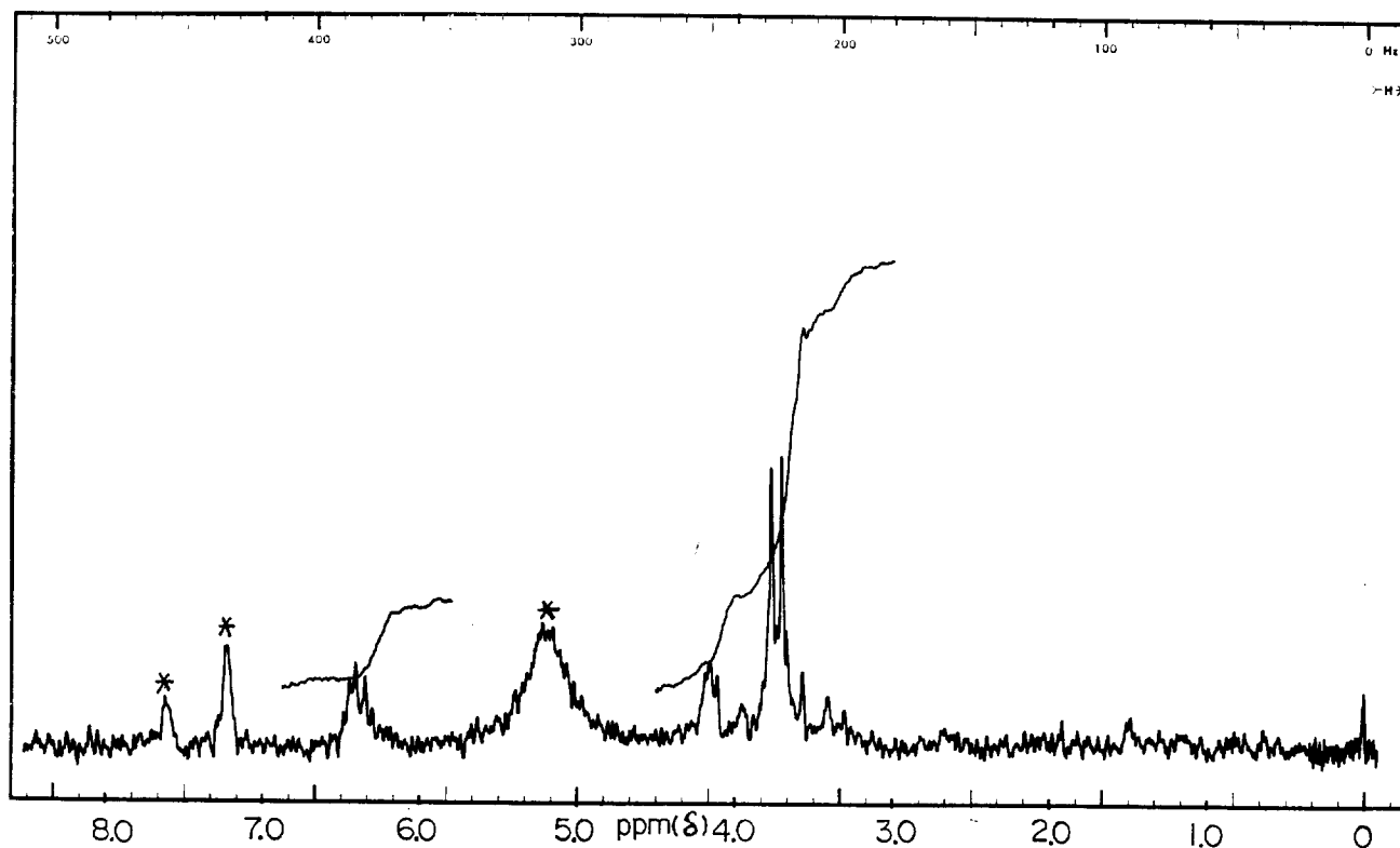
Figure 2. ^1\text{H} NMR spectrum of DMC-maleimide photoadduct (pyridine- d_5 ) ×: solvent peak.
