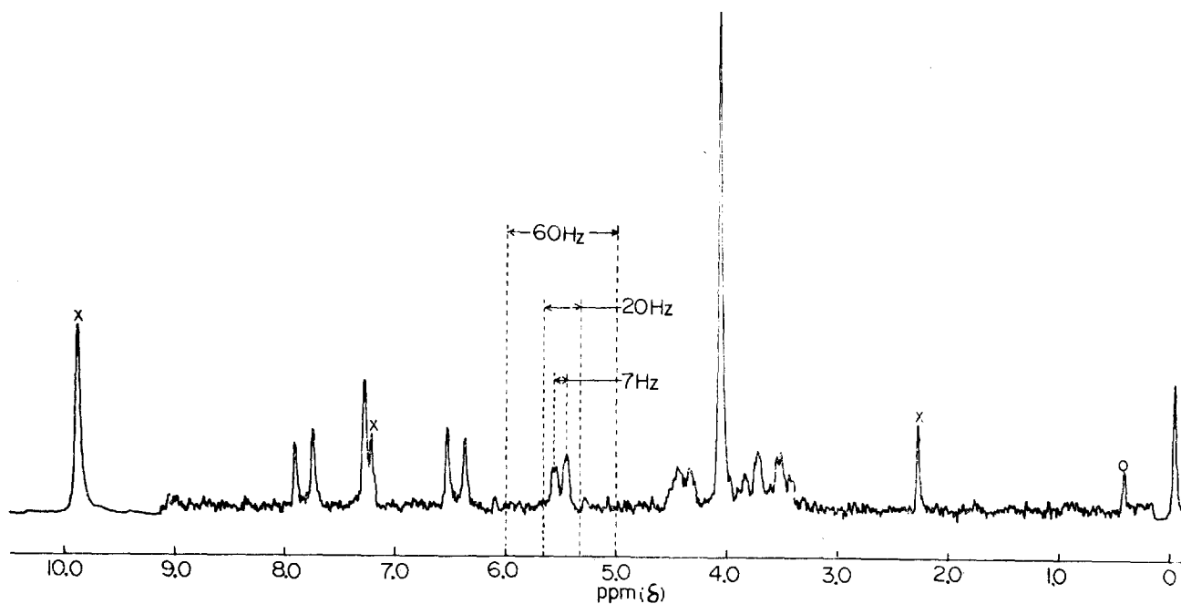
Figure 1. ^1\text{H} NMR spectrum of 8-MOP-maleimide photoadduct (chloroform- d /CF _3 COOH). X: solvent peak o: impurity.
