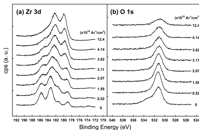
Figure 1. XP spectra of the Zr3d (a) and O1s (b) of D 2 O exposed to Zircaloy-4 surfaces after different Ar + fluences.
