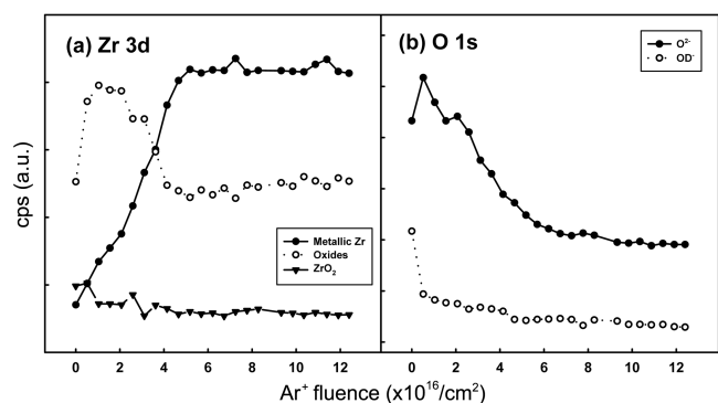
Figure 3. The relative ratios of the Zr3d (a) and O1s (b) peaks of the surface of D 2 O exposed to Zircaloy-4 as a function of the Ar + fluence.
