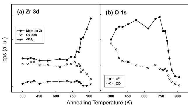
Figure 6. The relative ratios of the Zr3d (a) and O1s (b) peaks of the surface of D 2 O exposed to Zircaloy-4 as a function of annealing temperature.
