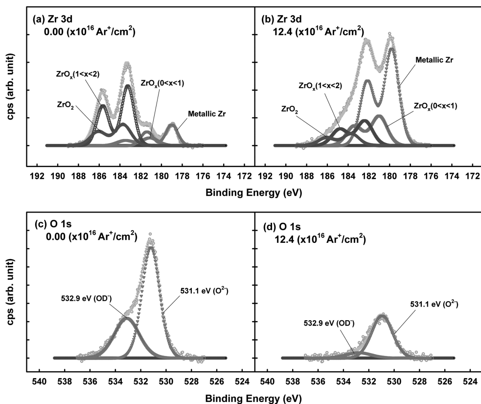
Figure 2. Deconvolution of measured Zr3d and O1s spectra of the D 2 O exposed to Zircaloy-4 after different Ar + fluences (a) Zr3d; 0.00 \times 10^{16} \text{Ar}^+/\text{cm}^2 (b) Zr3d; 12.4 \times 10^{16} \text{Ar}^+/\text{cm}^2 , (c) O1s; 0.00 \times 10^{16} \text{Ar}^+/\text{cm}^2 (d) O1s; 12.4 \times 10^{16} \text{Ar}^+/\text{cm}^2 .
