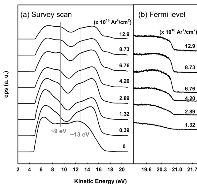
Figure 7. UP spectra of D 2 O exposed Zircaloy-4 after Ar-ion sputtering (a) survey scan and (b) high resolution UP spectra near Fermi level.
