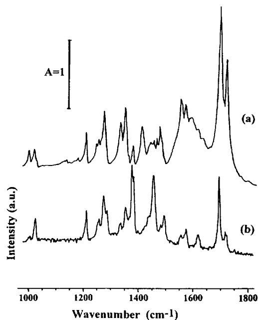
Figure 2. (a) FT-IR spectrum of lumichrome in solid phase at spectral resolution 4 cm -1 , coadding 100 times, in vacuo mode recorded using a Bomen DA 3.002 spectrophotometer equipped with a liquid Nitrogen-cooled MCT detector, a globar light source, and a KBr beam splitter (b) FT Raman spectrum of lumichrome in solid phase at spectral resolution 4 cm -1 , coadding 1000 times, laser power 0.1 W at sample, recorded using the same machine as above but equipped with liquid nitrogen-cooled InGaAs detector, 1064 nm excitation source from a Quantronix continuous-wave Nd:YAG laser, a quartz beam splitter, and a back-scattering collection optics system. (A: Absorbance, a.u.: arbitrary unit)
