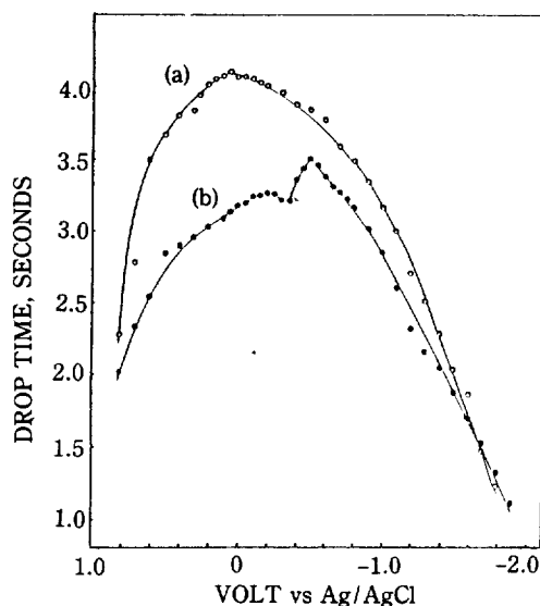
Figure 2. The electrocapillary curves (DME at h = 68 cm) of (a) 0.1 M Et_4NClO_4 in acetone (o) and (b) solution (a) plus 10^{-3} M mpno (●).
