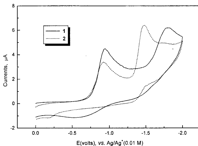
Figure 1. Cyclic voltammograms for \sim 1 \times 10^{-3} M (PyH) [MoOCl 2 (Sabp)](1) and (PyH)[MoO(NCS) 2 (Sabp)](2) in 0.1 M TEAP-DMSO (scan rate 100 mVs -1 ).
