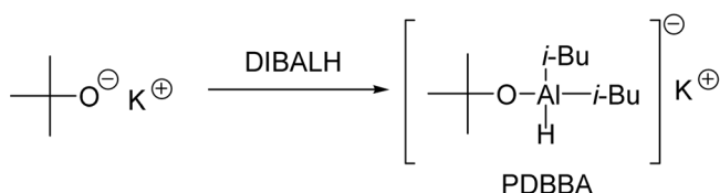
Scheme 1. Preparation of PDBBA.
