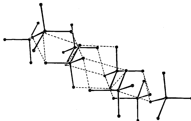
Figure 2. Crystal packing diagram of Li(bzac)(H 2 O) 2 showing the intermolecular hydrogen bonding along the z axis. Only Li and four oxygen atoms are shown for clarity.
