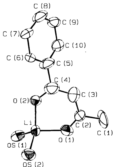
Figure 1. ORTEP drawing of the crystal structure of Li(bzac)(H 2 O) 2 showing the atomic labelling scheme and thermal ellipsoidal at 50% level.
