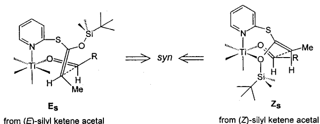
Figure 1. Titanium Mediated Chelation Transition State.
