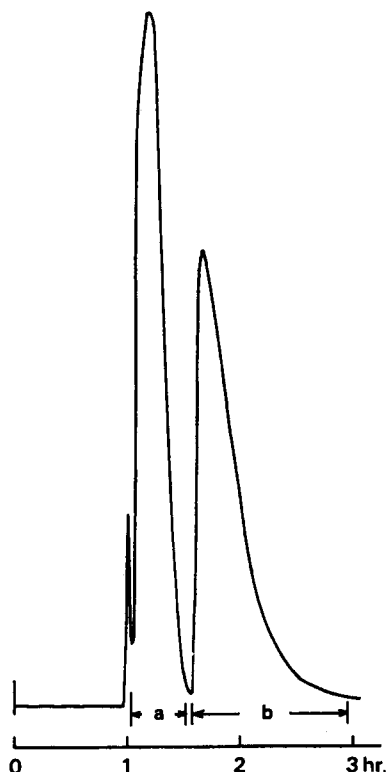
Figure 1. A representative MPLC chromatogram for separating the two enantiomers of 2.0 g of racemic compound 2 on CSP 1 . See experimental part for the chromatographic conditions. The two fractions corresponding to the two enantiomers were collected within the marked duration a and b .
