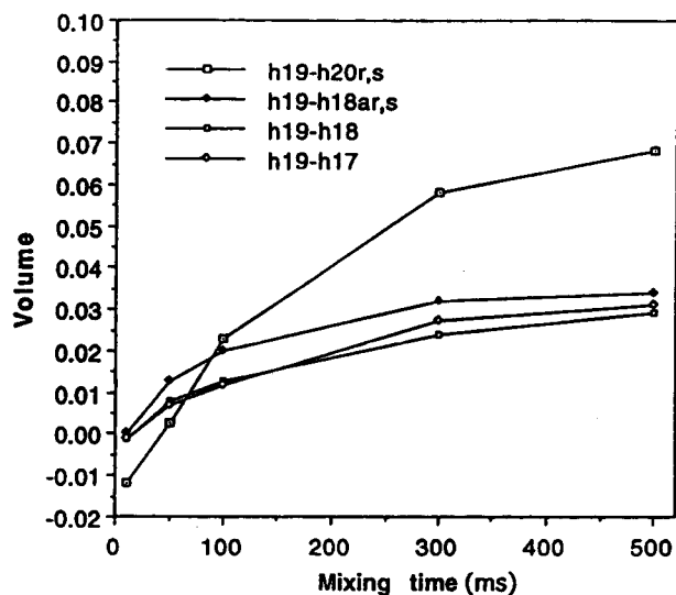
Figure 4. NOE buildup curves from H19 to neighboring protons. Severe correlated spectroscopy (COSY) effect were appeared on H19-H20r,s at lower mixing time (10-100 ms) due to the contribution of both through bond and through space coupling. Negative NOEs and fast slope of NOE buildup is in general from COSY effect.
