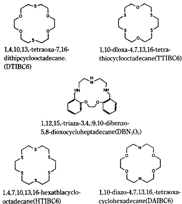
Figure 2. Macrocylic ligands used in this study.
