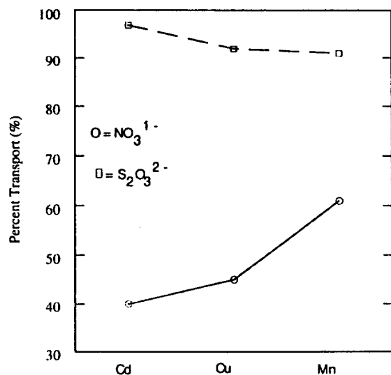
Figure 5. Single transport of several \text{M}^{2+} in emulsion liquid membrane as a kind of \text{NO}_3^- or \text{S}_2\text{O}_3^{2-} in the receiving phase by \text{DBN}_3\text{O}_2 .
