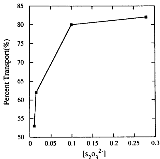
Figure 4. Transport of \text{Cu}^{2+} in emulsion liquid membrane as a function of \text{S}_2\text{O}_3^{2-} concentration in receiving phase by \text{DBN}_3\text{O}_2 .
