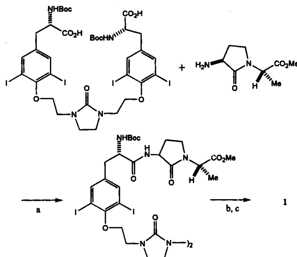
Scheme 1. (a) DCC/HOBT (78%), (b) i. NaOH, ii. C 6 F 5 OH/EDC (45%), (c) DIPEA, THF (35%).
