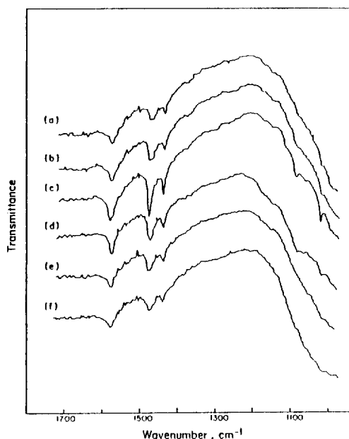
Figure 1. Infrared spectra of benzenethiol on silver at pressures of 90 mTorr (a), 150 mTorr (b), and 1 Torr (c), followed by evacuation for 1 hr at 300 K (d), 573 K (e), and 673 K (f).
