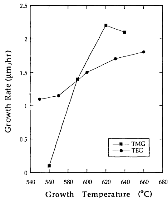
Figure 2. Effect of growth temperature on the GaAs growth rates using unprecracked MEAs with TMG ( V/\text{III}=10 , P=5.5 \times 10^{-5} Torr) and TEG ( V/\text{III}=20 , P=5.7 \times 10^{-4} Torr).
