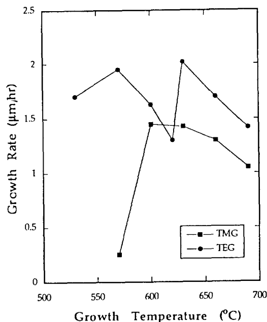
Figure 1. Effect of growth temperature on the GaAs growth rates using unprecracked \text{AsH}_3 with TMG ( V/\text{III}=10 , P=1.2 \times 10^{-4} Torr) and TEG ( V/\text{III}=20 , P=1.2 \times 10^{-4} Torr).
