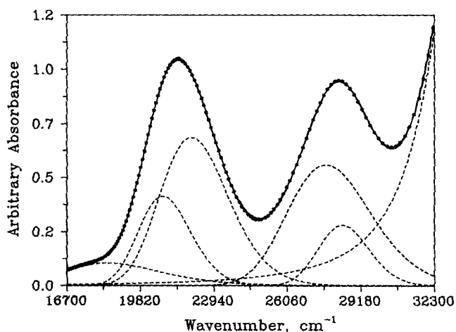
Figure 4. Electronic absorption spectrum of [\text{Cr}(\text{NH}_3)_5(\text{imH})]^{3+} in aqueous solution at 298 K.
