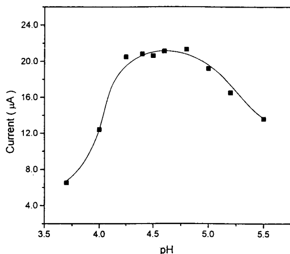
Figure 3. Effect of pH on the peak current of cyclic voltammograms for 2.0 \times 10^{-5} M cobalt(II) solution obtained using 20% PAN modified carbon paste electrode: preconcentration time, 8 min at 43 °C; reduction time, 1 min; scan rate, 50 mV/s.
