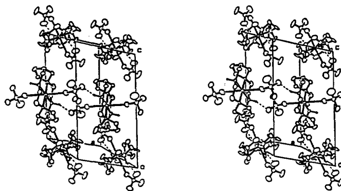
Figure 2. A stereoscopic packing diagram. Two complexes in the middle of the figure are B and the other four complexes are A. The O atoms of the perchlorate B in the minor sites and the H atoms except those for the hydrogen bonds are omitted for clarity. The dashed lines denote the hydrogen bonds.
