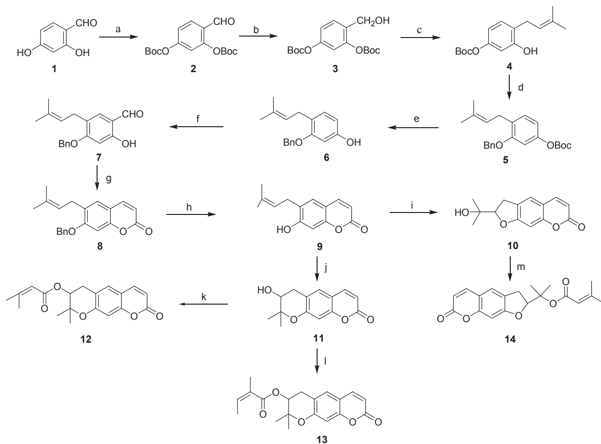
Scheme 1. Synthesis of Marmesin, Decursinol and their analogues. Reaction Conditions: (a) (\text{Boc})_2\text{O} , \text{K}_2\text{CO}_3 , ether, rt, 90%; (b) \text{NaBH}_4 , THF, conc HCl, AcOH, 0^\circ\text{C} , 15 min, 70% (c) 2-methyl-1-propenyl magnesium bromide, THF, 0^\circ\text{C} to rt, 10 h, 71% (d) \text{BnBr} , \text{K}_2\text{CO}_3 , DMF, rt, 12 h, 81% (e) 1M HCl in dioxane, MeOH, rt, 91% (f) \text{CH}(\text{OEt})_3 , \text{AlCl}_3 , benzene, rt, 30 min, 48% (g) (carbethoxymethylene)triphenylphosphorane, N,N -diethyl aniline, 190^\circ\text{C} , 5 h, 89% (h) Raney Ni, EtOH, rt, 3 h, 90% (i) m -chloroperbenzoic acid, \text{NaHCO}_3 , \text{CHCl}_3 , \text{NaHSO}_3 , NaOH, 0^\circ\text{C} to rt, 3 h, 80% (j) m -chloroperbenzoic acid, p -toluenesulfonic acid, \text{CHCl}_3 , rt, 12 h, 72% (k) DCC, angelic acid, DMAP, rt, 26 h, 38% (l) LiHMDS, DMAP, seneciyl chloride, -40^\circ\text{C} , 18 h, 36% (m) DCC, angelic acid, 30^\circ\text{C} , 24 h, 48%
